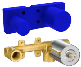
Available in ● ● ● ● NOB-0708 Body of Single Lever Wall Mounted Concealed Basin Mixer consisting of Cartridge, Cartridge Sleeve & Protective Cover
